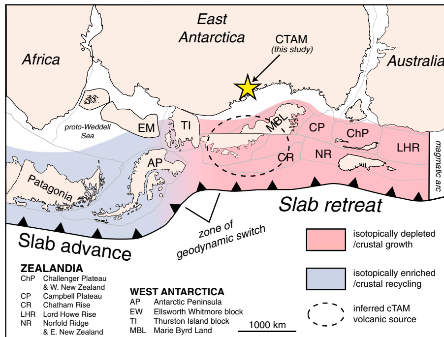
Figure 9. Reconstruction of the Gondwana plate margin, approximately Permian (Elliot, 2013). Shown are the inferred limits of the continuous retreating arc system that is isotopically depleted (red) and the advancing arc system that is isotopically enriched (blue). The zone of the geochemical and geodynamic switch occurs in the vicinity of the Thurston Island block. The region outboard of the cTAM is interpreted to be the isotopically depleted arc source for volcanoclastic sediments of the cTAM.
