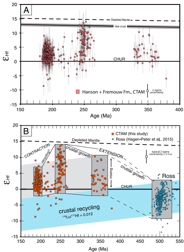
Figure 6. (a) Zircon age versus initial \epsilon_{Hf} plot summarizing all Hf isotopic data from this study. (b) Hf isotopic data from this study combined with data for the Ross Orogen from Hagen-Peter et al. (2015) and the inferred geodynamic evolution of the Antarctic sector arc system. Inclined gray and blue fields correspond to hypothetical fields of crustal recycling assuming a Lu/Hf = 0.012 (Rudnick & Gao, 2003). Hf isotopic values for depleted mantle and new crust are from Vervoort and Blichert-Toft (1999) and Dhuime et al. (2011). CHUR, chondritic uniform reservoir. See Data Set S2 for full zircon Hf isotope data set.
