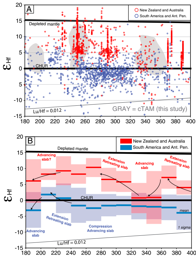
Figure 8. (a) Compilation of zircon Hf isotope data from Australia-Zealandia (red) and South America-Antarctica Peninsula (blue). Fields for Hf isotope data from the cTAM (this study) are provided in gray. Data for Australia-Zealandia are from Veevers et al. (2006), Li et al. (2015), Shaw et al. (2011), Phillips et al. (2011), Kemp et al. (2009, 2007, 2005), Jeon et al. (2014), Regmi et al. (2016), Murgulov et al. (2007), Nebel et al. (2007), Hiess et al. (2015), Scott et al. (2009), and Milan et al. (2016). Data from South America-Antarctica Peninsula are from Bahlburg et al. (2009), Flowerdew et al. (2006), Bradshaw et al. (2012), Castillo et al. (2015), Fanning et al. (2011), Pepper et al. (2016), Rey et al. (2016), Pankhurst et al. (2016), and Canile et al., 2016. (b) Mean and 1 sigma uncertainty for data from Figure 8a grouped into 20 Myr bins, and the inferred intervals of increasing or decreasing initial \epsilon_{\text{Hf}} combined with geodynamic interpretations. Hf isotopic values for depleted mantle and new crust are from Vervoort and Blichert-Toft (1999). CHUR, chondritic uniform reservoir.
